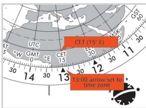
Fig. 7: Setting the time zone
