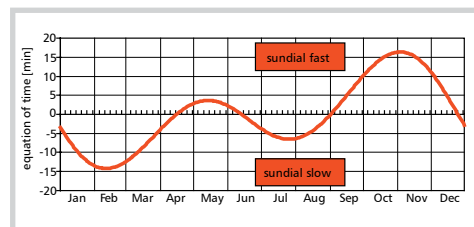
Fig. 2: Equation of time
