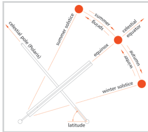
Fig. 4: Seasons
